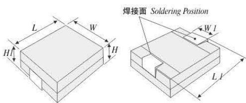
➤ Fig.1 Structure and dimension of inward(C style) Chip Zinc Oxide Varistor
