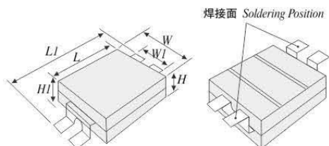
Fig.2 Structure and dimension of outward(Y style) Chip Zinc Oxide Varistor
